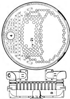
Figs. 490-490. Headers for Cole Superheater.
